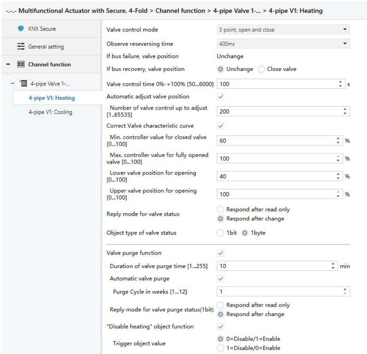
Fig. 4.9.1.3 Parameter window "3 point, open and close"
