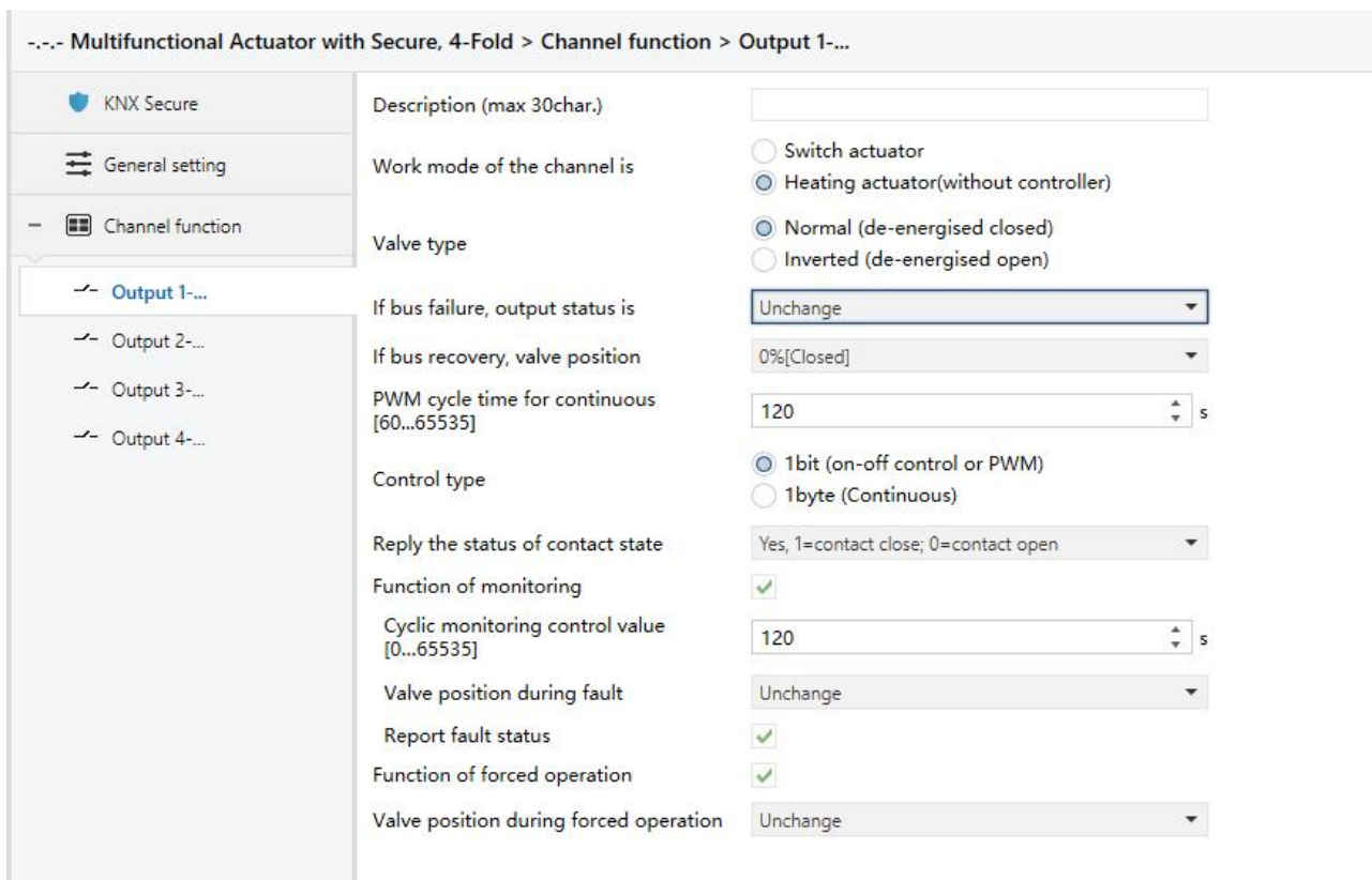
Fig. 4.5(1) Parameter window “Output X: Heating actuator(without controller)_1bit (on-off control or PWM) ”
