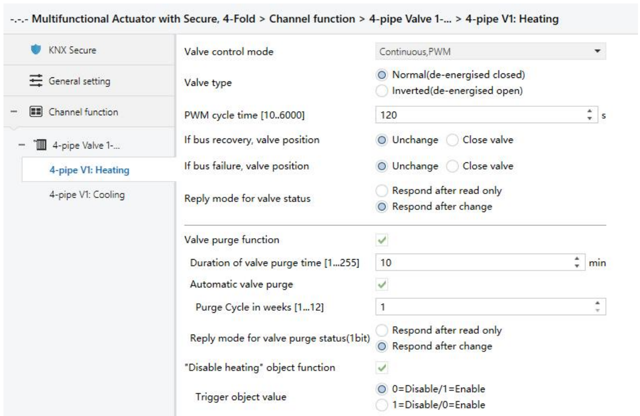
Fig. 4.9.1.2 Parameter window "Continuous, PWM"
