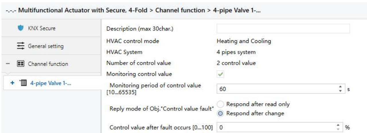
Fig. 4.9(5) Parameter window “4-Pipe Valve X General–Heating and Cooling (4-pipes)”
