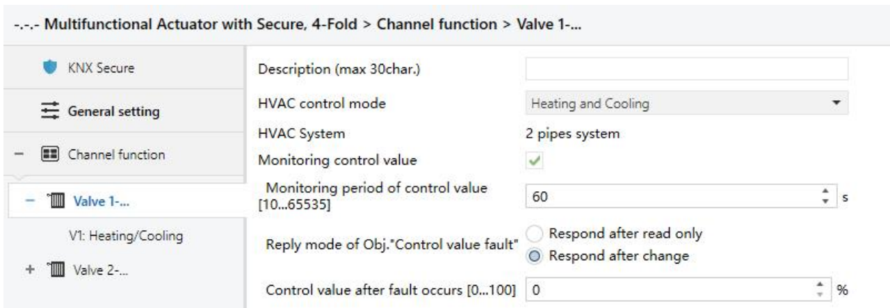
Fig. 4.9(4) Parameter window “Valve X General–Heating and Cooling (2-pipes)”
