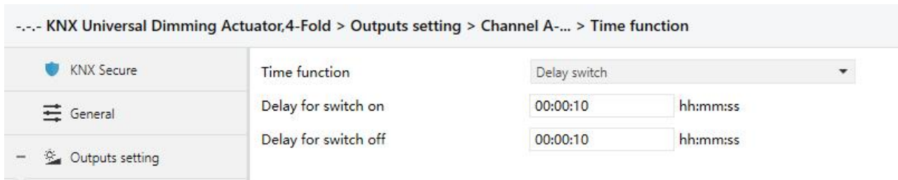
Delay switch
