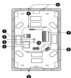
Input connection
