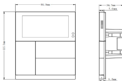
Panel dimension
