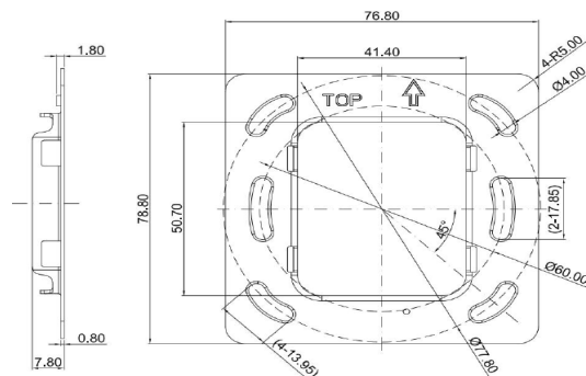
Metal plate dimension
