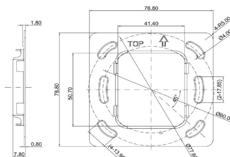
Metal plate dimension
