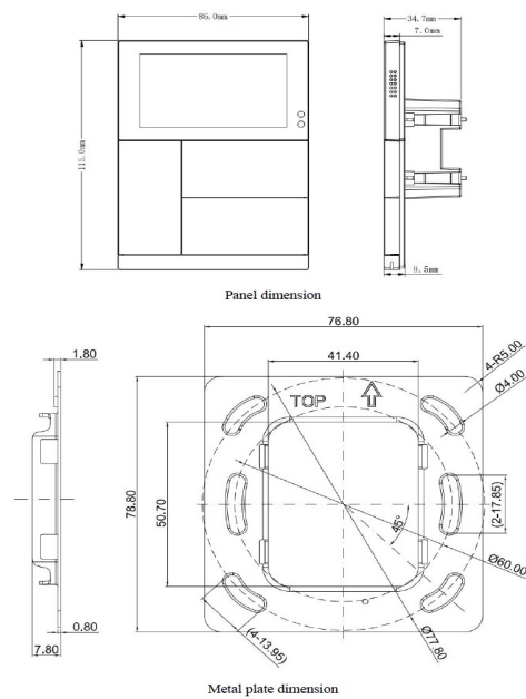
3.1 Dimension Diagram
