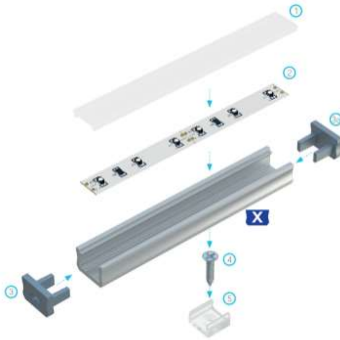
Assembly scheme for elements of the lighting system using profile X and (1) a SLIM cover, (2) a LED strip, (3) an end cap with hole, (3a) an end cap without hole, (4) a mounting screw, (5) a mounting clip X
