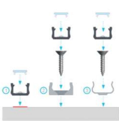
Installation instructions for profile X with a GUM cover using (1) a double-sided tape, (2) a mounting clip X and (3) a metal mounting clip X
