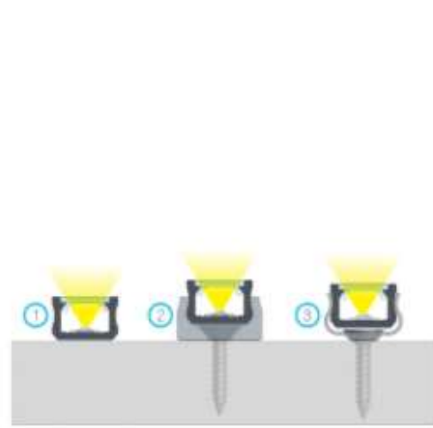
The end result of installation of profile X with a GUM cover using (1) a double-sided tape, (2) a mounting clip X and (3) a metal mounting clip X
