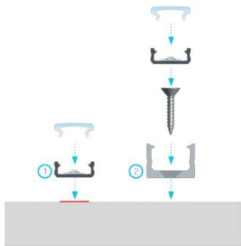
Installation instructions for profile D with a HIGH cover using (1) a double-sided tape, (2) a D HIGH mounting clip
