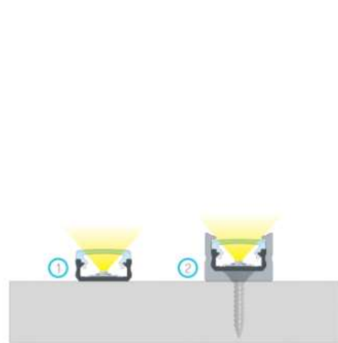
The end result of installation of profile D with a HIGH cover using (1) a double-sided tape, (2) a D HIGH mounting clip
