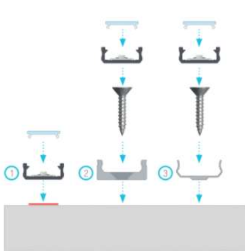
Installation instructions for profile D with a BASIC cover using (1) a double-sided tape, (2) a D MINI mounting clip and (3) a metal D mounting clip
