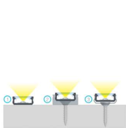
The end result of installation of profile D with a BASIC cover using (1) a double-sided tape, (2) a D MINI mounting clip and (3) a metal D mounting clip
