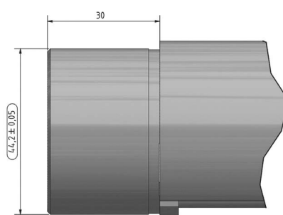
Fig. Adapter on round tube 48.3 x 3 mm
